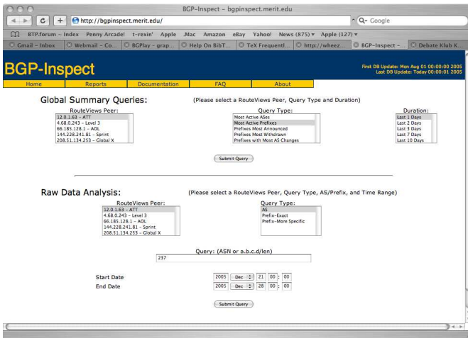
Fig. 3. BGP-Inspect Query Interface
