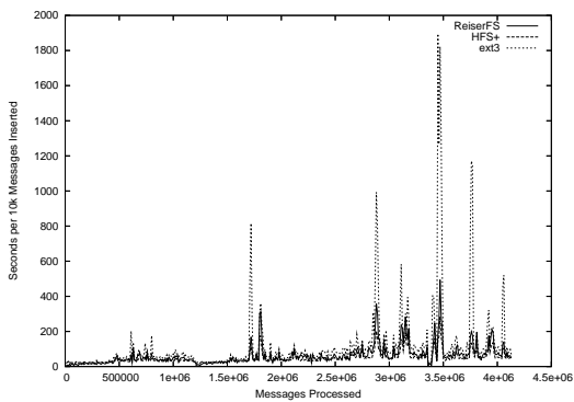
Fig. 9. Database Speed vs. File System
