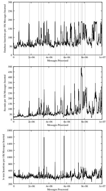
Fig. 8. Correlation between Insertion count and Processing Time
