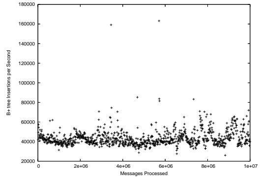
Fig. 7. B+ tree Insertions over time
