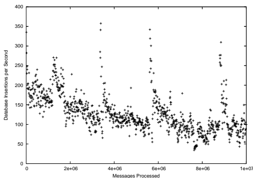
Fig. 10. Database Insertions over time
