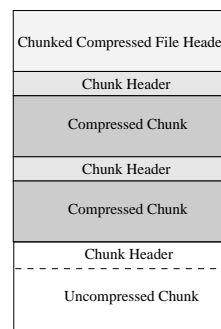
Fig. 2. Chunked Compressed File Structure
