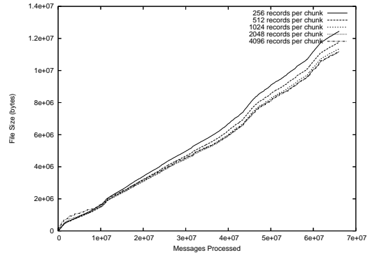
Fig. 6. Chunk Sizes vs. File Size
